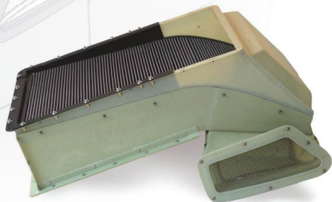
Legacy EC130 Design
